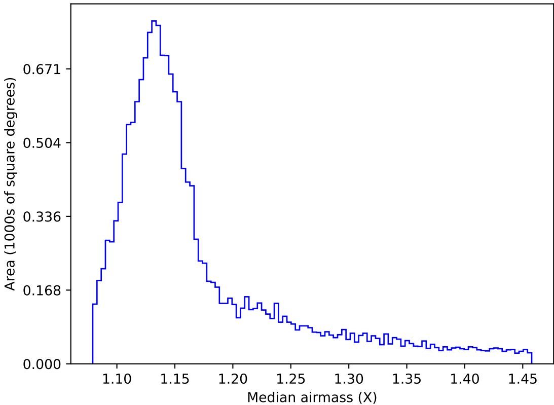
too_elab_r8_d3_giz_v3.4_10yrs WFD i band: Median airmass
