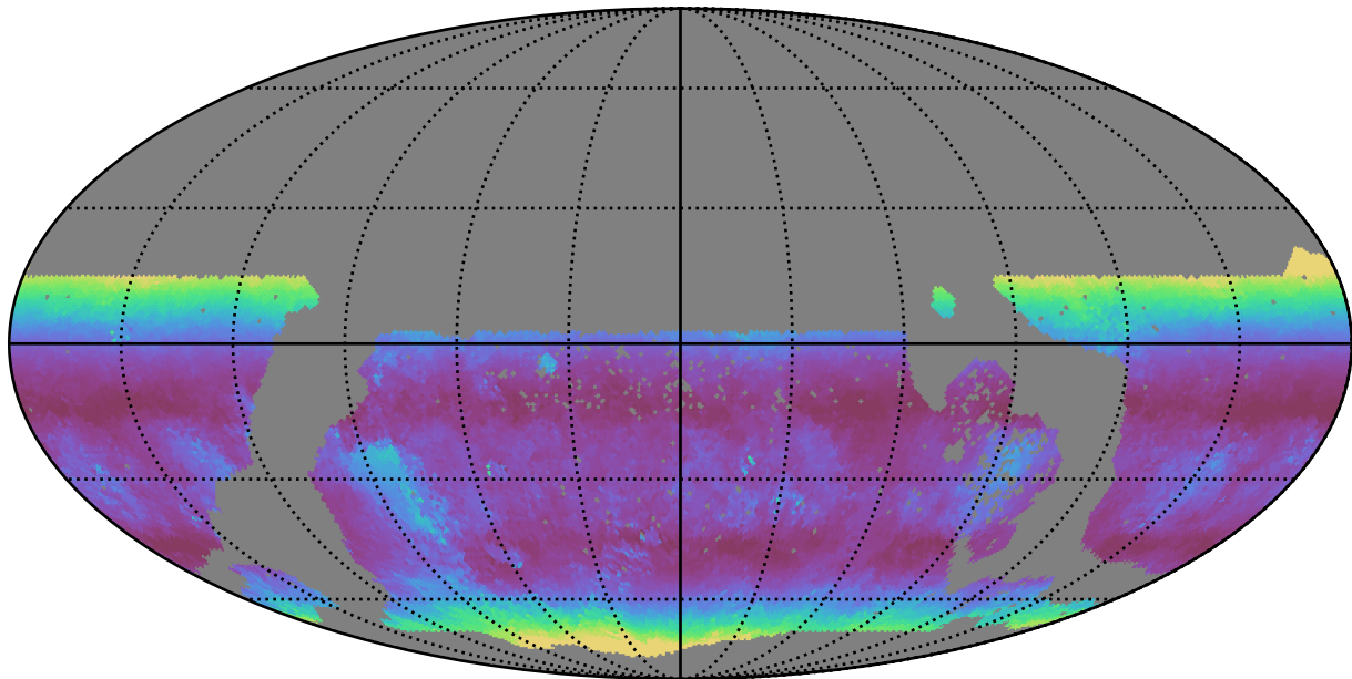
too_elab_r8_d3_giz_v3.4_10yrs WFD g band: Median airmass
