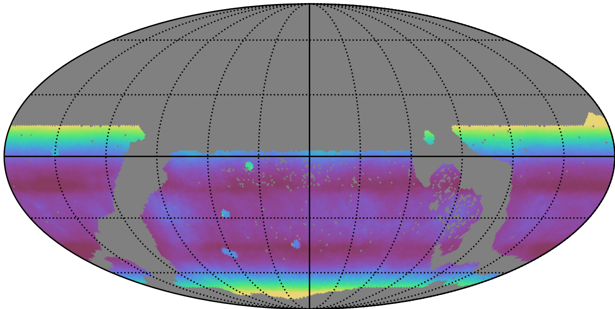
too_elab_r8_d3_giz_v3.4_10yrs WFD all bands: Median airmass
