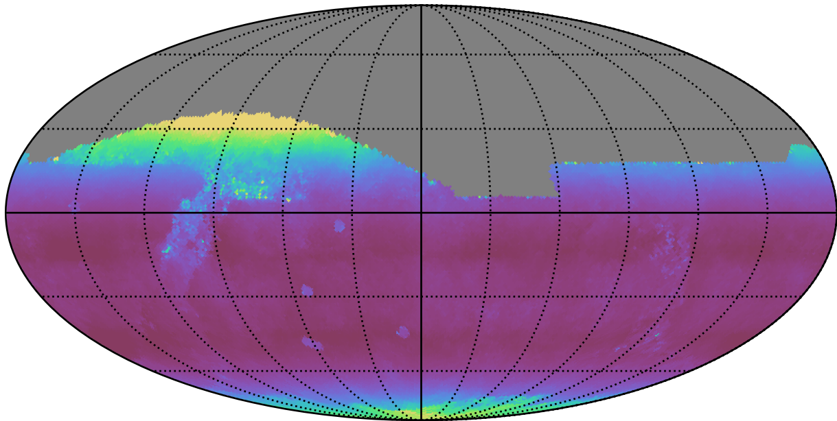
too_elab_r8_d3_giz_v3.4_10yrs All sky z band: Median airmass
