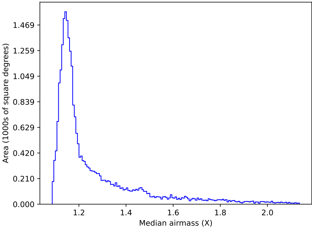
too_elab_r8_d3_giz_v3.4_10yrs All sky z band: Median airmass
