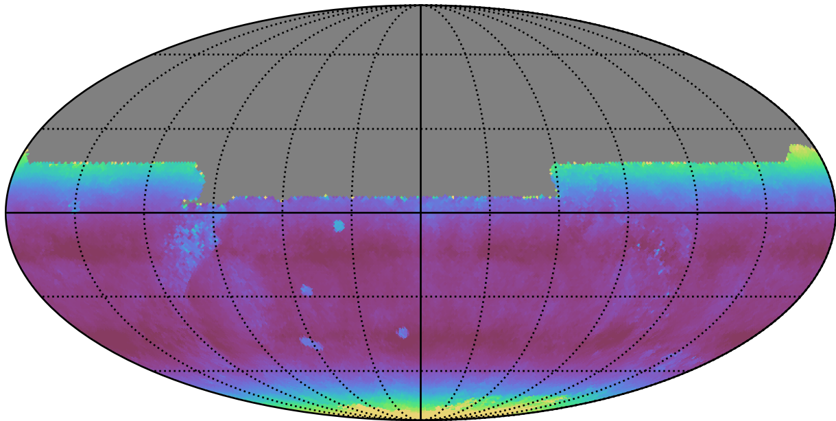
too_elab_r8_d3_giz_v3.4_10yrs All sky y band: Median airmass
