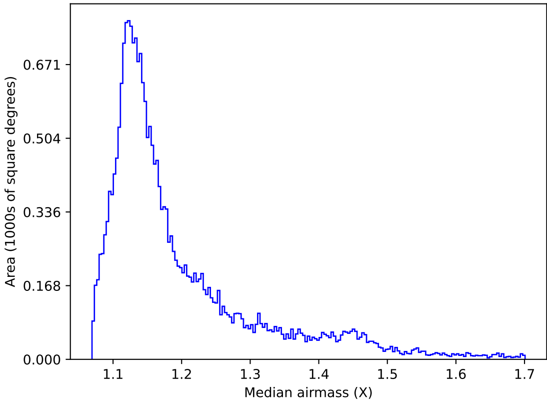
too_elab_r8_d3_giz_v3.4_10yrs All sky u band: Median airmass
