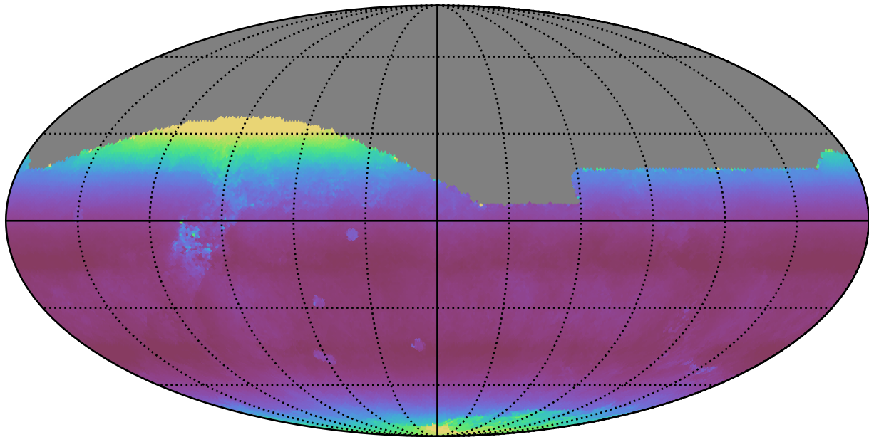
too_elab_r8_d3_giz_v3.4_10yrs All sky r band: Median airmass
