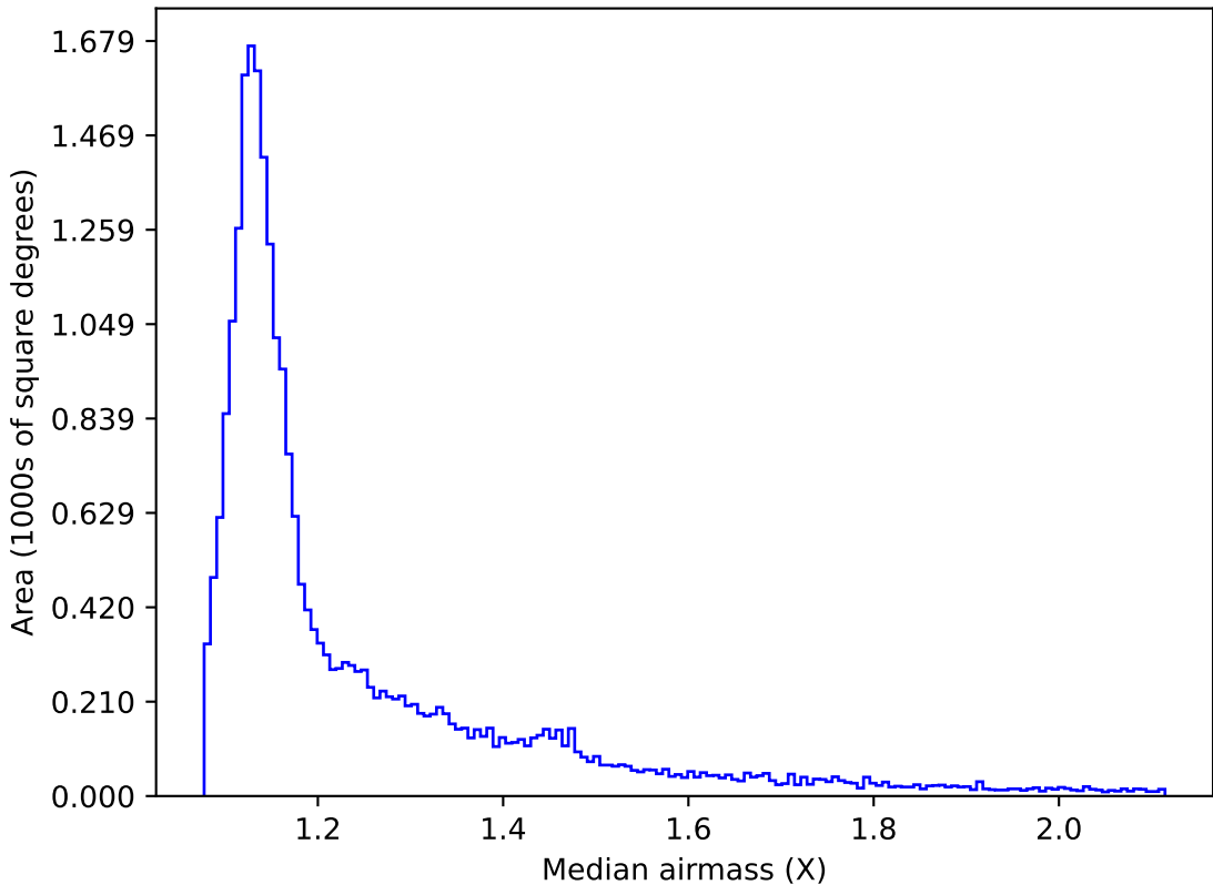
too_elab_r8_d3_giz_v3.4_10yrs All sky r band: Median airmass
