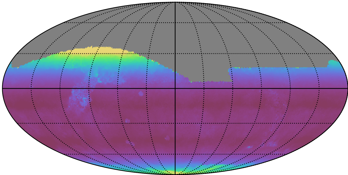
too_elab_r8_d3_giz_v3.4_10yrs All sky i band: Median airmass
