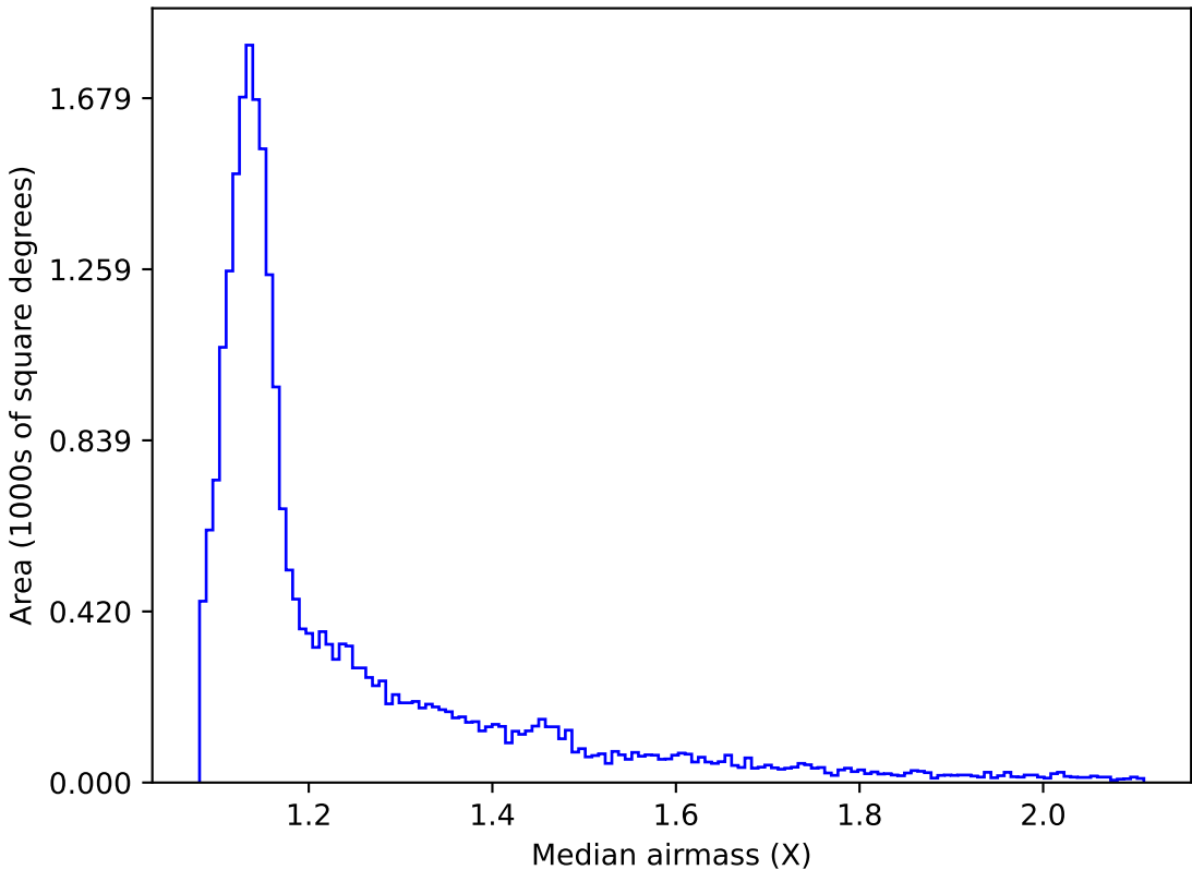
too_elab_r8_d3_giz_v3.4_10yrs All sky i band: Median airmass
