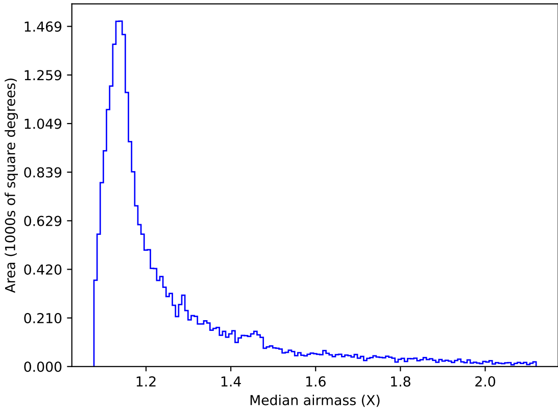
too_elab_r8_d3_giz_v3.4_10yrs All sky g band: Median airmass
