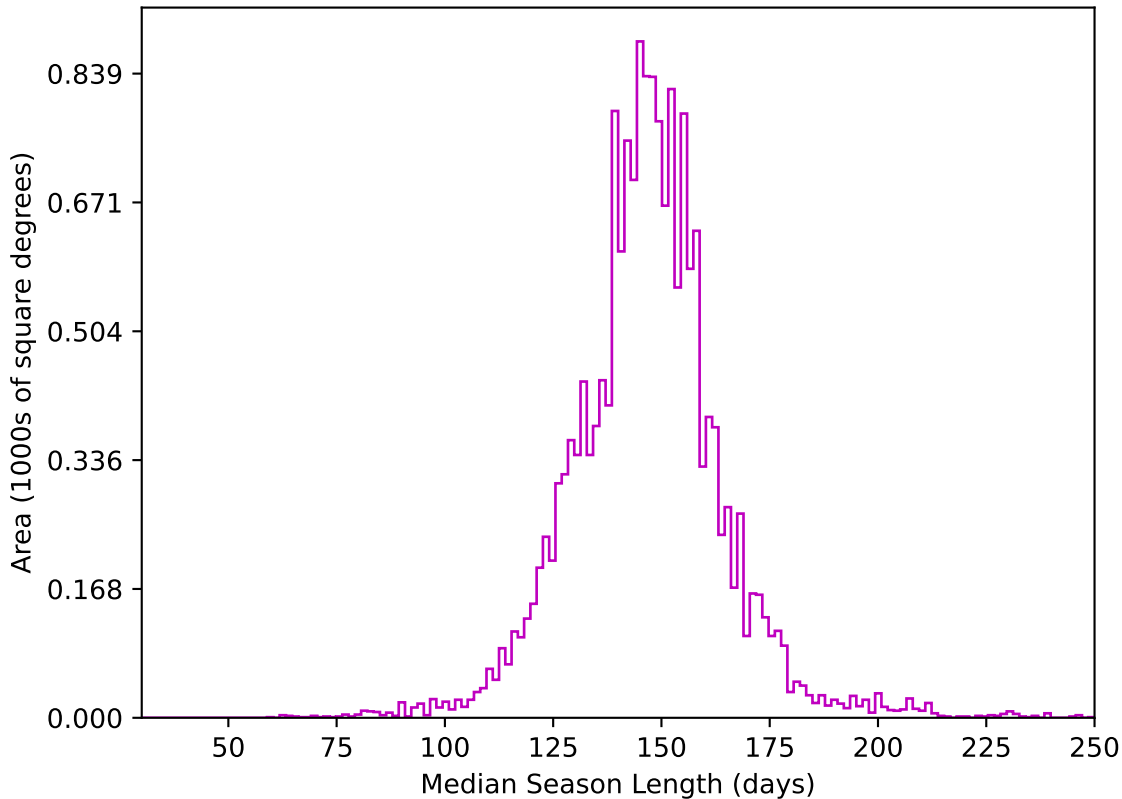
too_elab_r8_d3_giz_v3.4_10yrs WFD z band: Median Season Length
