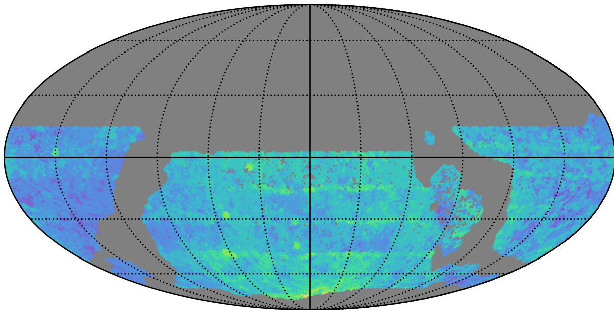
too_elab_r8_d3_giz_v3.4_10yrs WFD y band: Median Season Length
