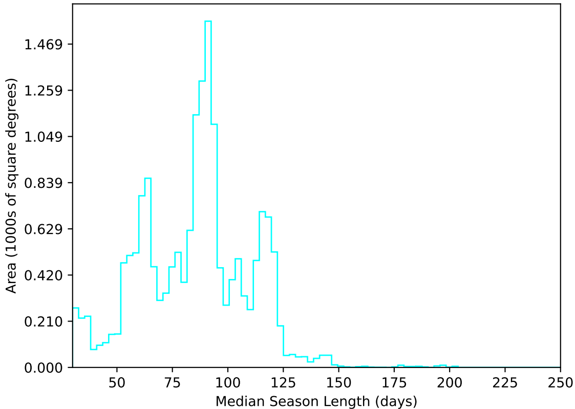
too_elab_r8_d3_giz_v3.4_10yrs WFD u band: Median Season Length
