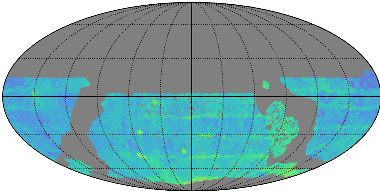
too_elab_r8_d3_giz_v3.4_10yrs WFD r band: Median Season Length
