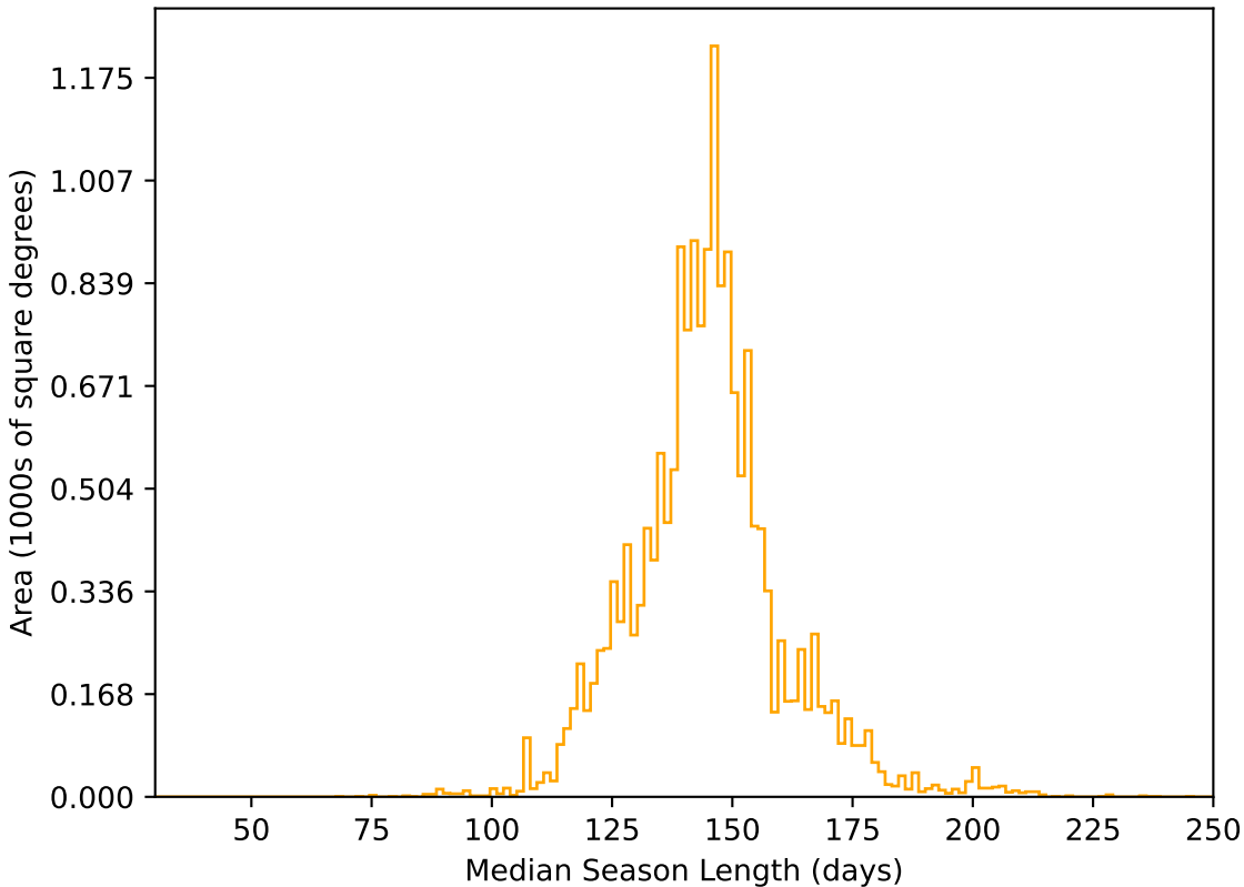
too_elab_r8_d3_giz_v3.4_10yrs WFD r band: Median Season Length
