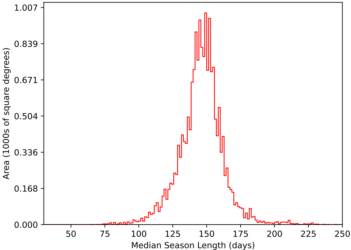
too_elab_r8_d3_giz_v3.4_10yrs WFD i band: Median Season Length
