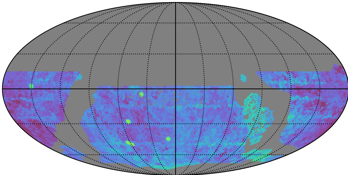
too_elab_r8_d3_giz_v3.4_10yrs WFD g band: Median Season Length
