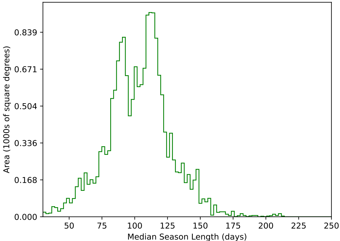
too_elab_r8_d3_giz_v3.4_10yrs WFD g band: Median Season Length
