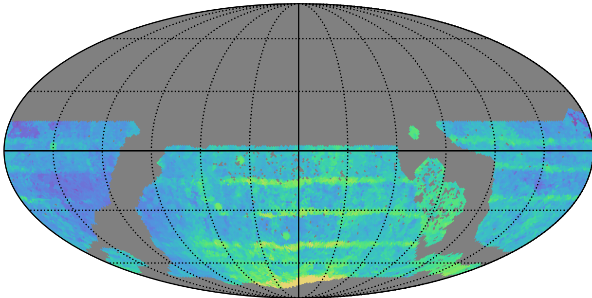
too_elab_r8_d3_giz_v3.4_10yrs WFD all bands: Median Season Length
