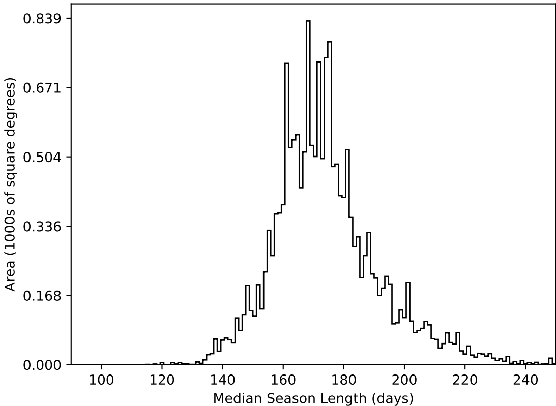
too_elab_r8_d3_giz_v3.4_10yrs WFD all bands: Median Season Length
