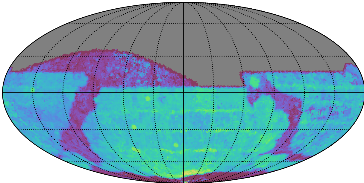
too_elab_r8_d3_giz_v3.4_10yrs All sky z band: Median Season Length
