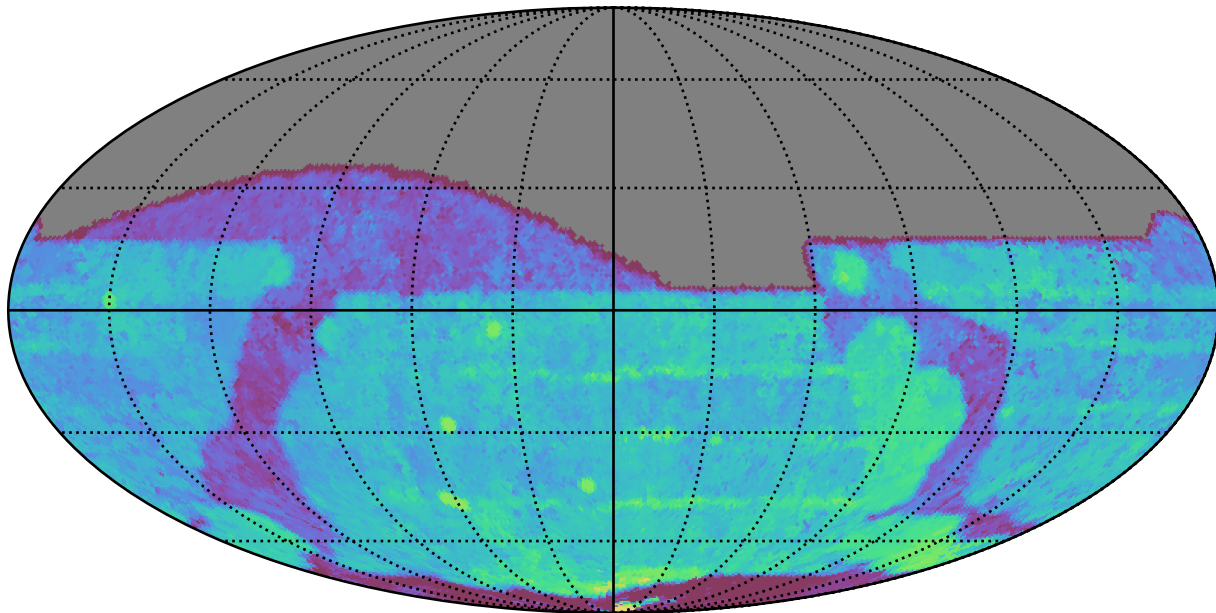
too_elab_r8_d3_giz_v3.4_10yrs All sky r band: Median Season Length
