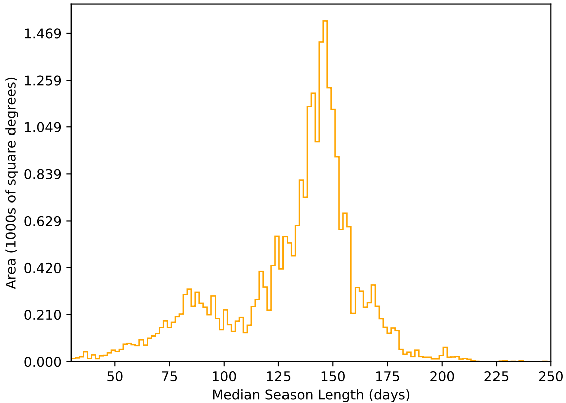
too_elab_r8_d3_giz_v3.4_10yrs All sky r band: Median Season Length
