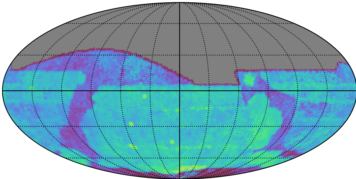
too_elab_r8_d3_giz_v3.4_10yrs All sky i band: Median Season Length
