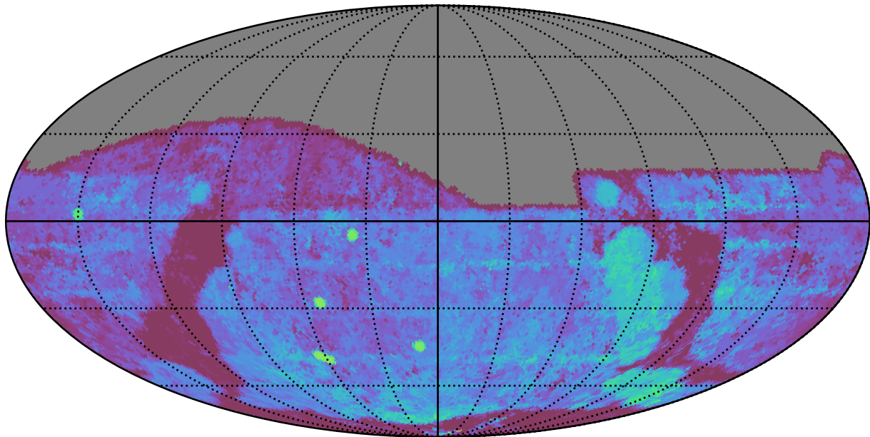
too_elab_r8_d3_giz_v3.4_10yrs All sky g band: Median Season Length
