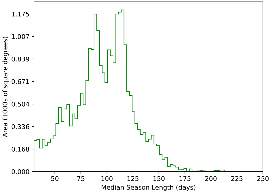
too_elab_r8_d3_giz_v3.4_10yrs All sky g band: Median Season Length
