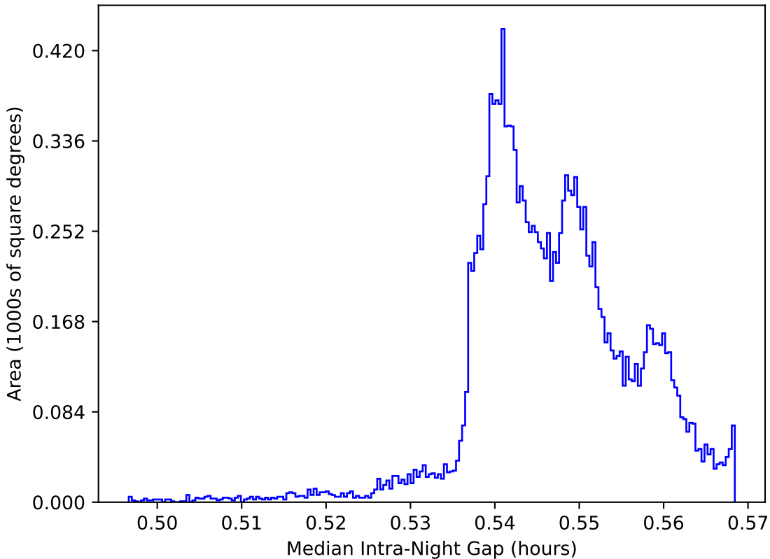
too_elab_r8_d3_giz_v3.4_10yrs WFD: Median Intra-Night Gap
