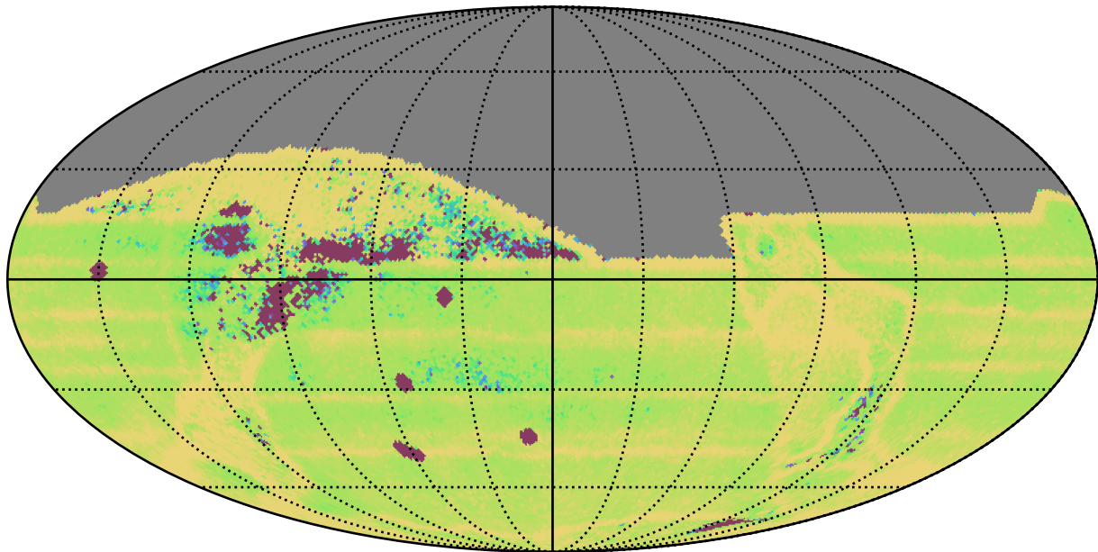
too_elab_r8_d3_giz_v3.4_10yrs All sky: Median Intra-Night Gap
