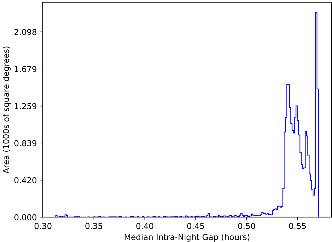
too_elab_r8_d3_giz_v3.4_10yrs All sky: Median Intra-Night Gap
