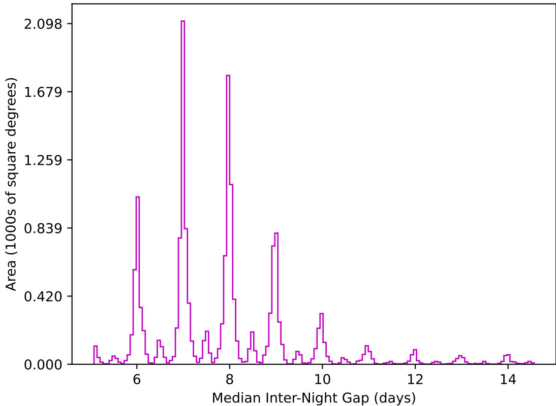
too_elab_r8_d3_giz_v3.4_10yrs WFD z band: Median Inter-Night Gap
