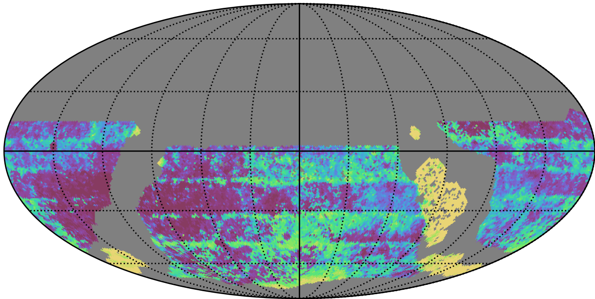
too_elab_r8_d3_giz_v3.4_10yrs WFD y band: Median Inter-Night Gap
