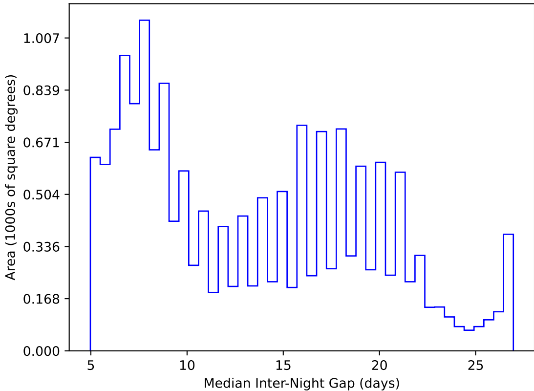
too_elab_r8_d3_giz_v3.4_10yrs WFD y band: Median Inter-Night Gap
