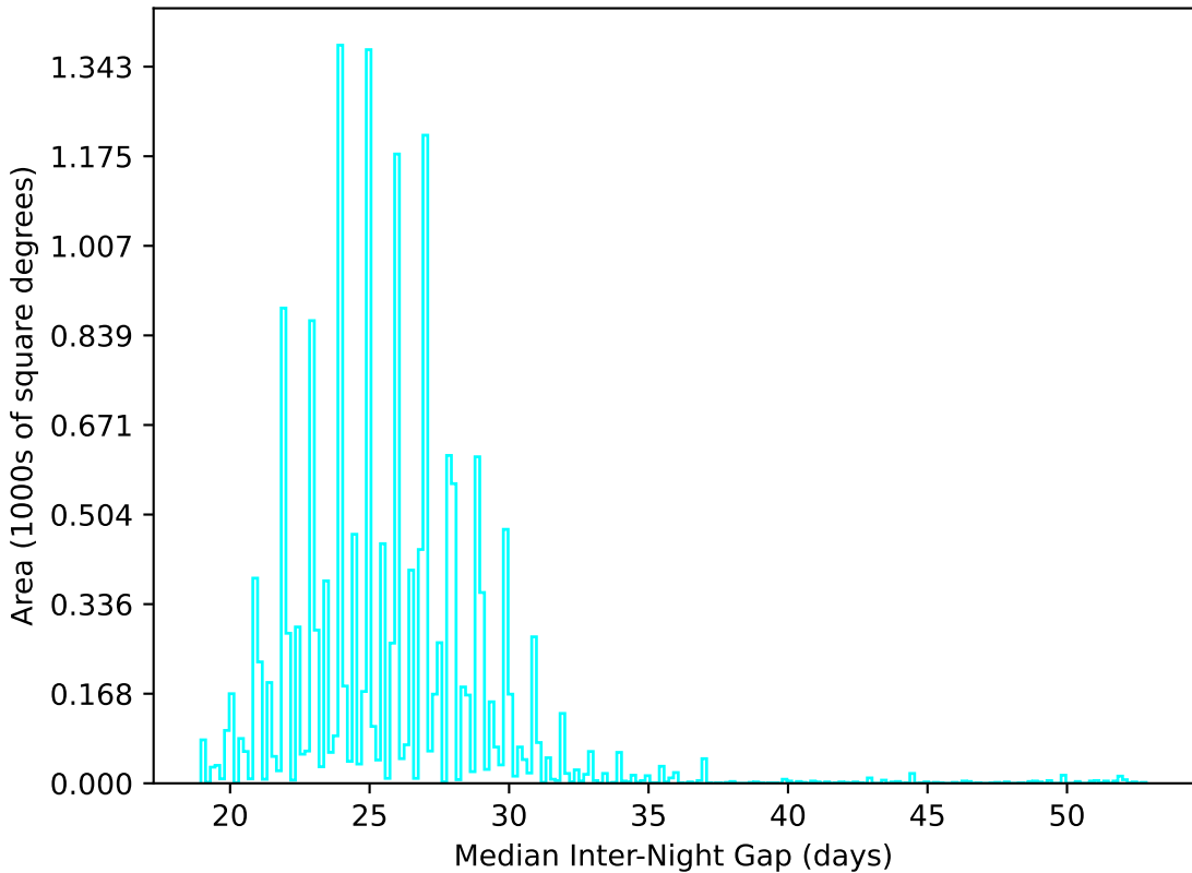
too_elab_r8_d3_giz_v3.4_10yrs WFD u band: Median Inter-Night Gap
