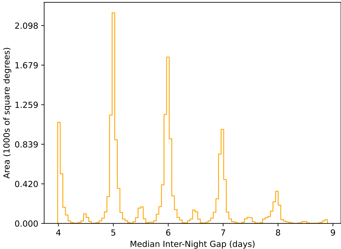
too_elab_r8_d3_giz_v3.4_10yrs WFD r band: Median Inter-Night Gap
