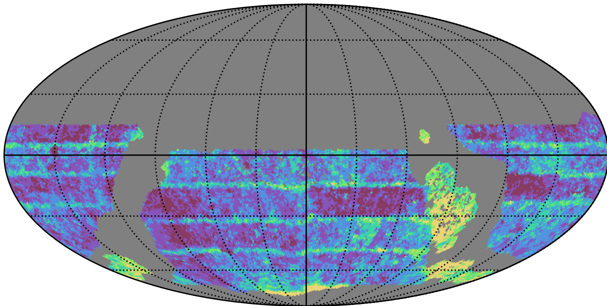
too_elab_r8_d3_giz_v3.4_10yrs WFD i band: Median Inter-Night Gap
