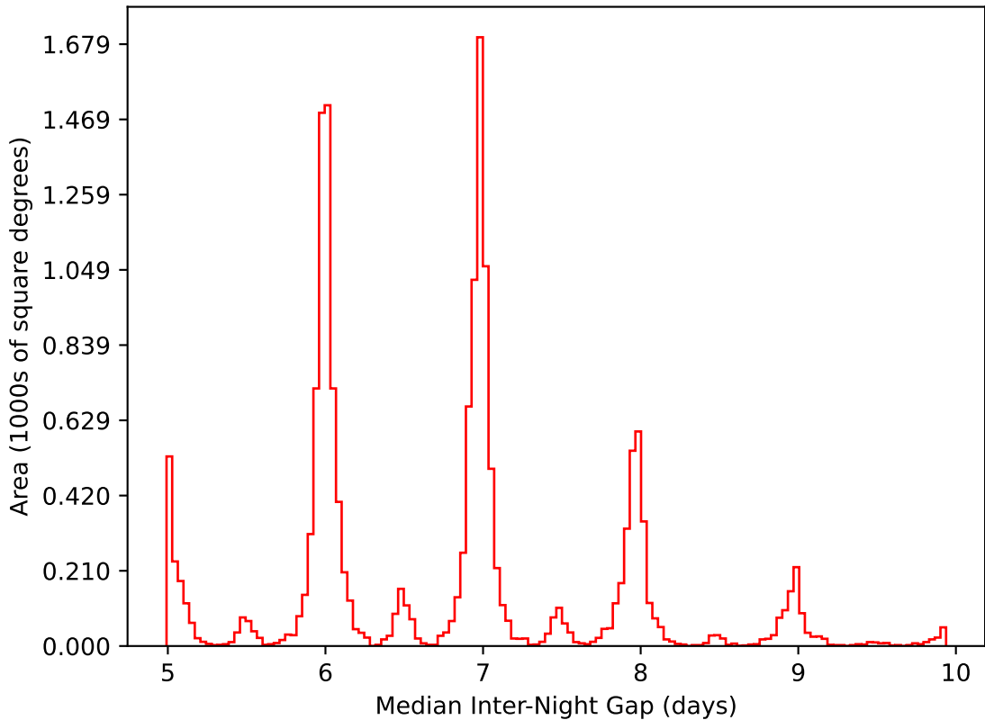
too_elab_r8_d3_giz_v3.4_10yrs WFD i band: Median Inter-Night Gap
