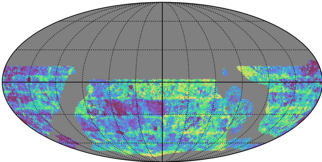
too_elab_r8_d3_giz_v3.4_10yrs WFD g band: Median Inter-Night Gap
