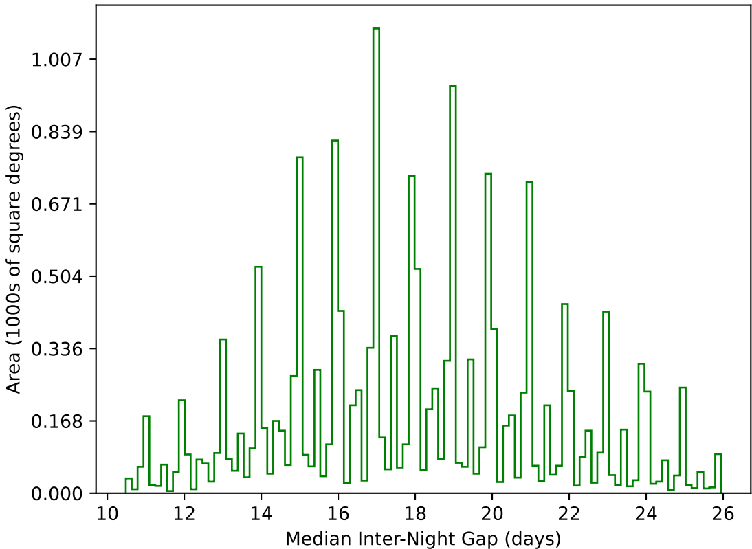
too_elab_r8_d3_giz_v3.4_10yrs WFD g band: Median Inter-Night Gap
