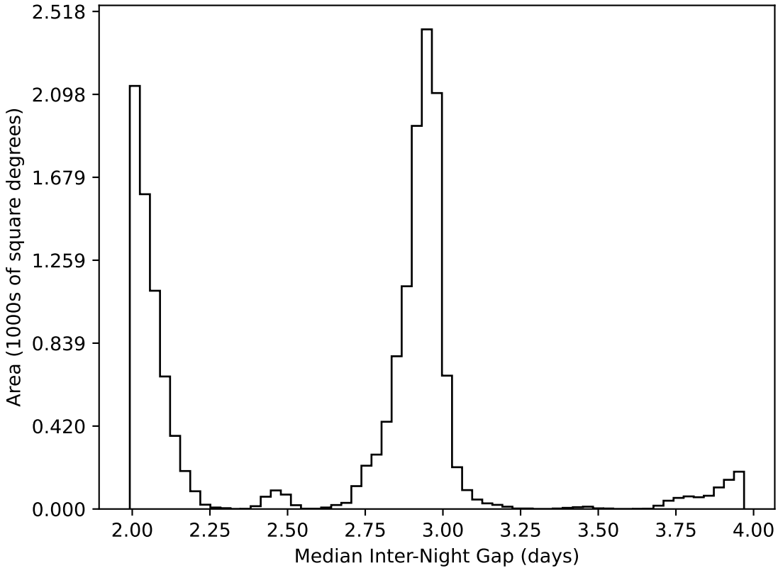
too_elab_r8_d3_giz_v3.4_10yrs WFD all bands: Median Inter-Night Gap
