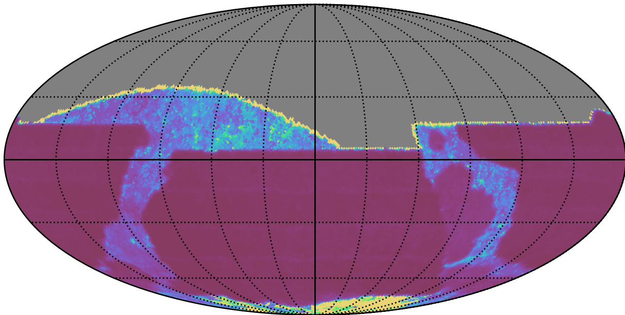
too_elab_r8_d3_giz_v3.4_10yrs All sky z band: Median Inter-Night Gap
