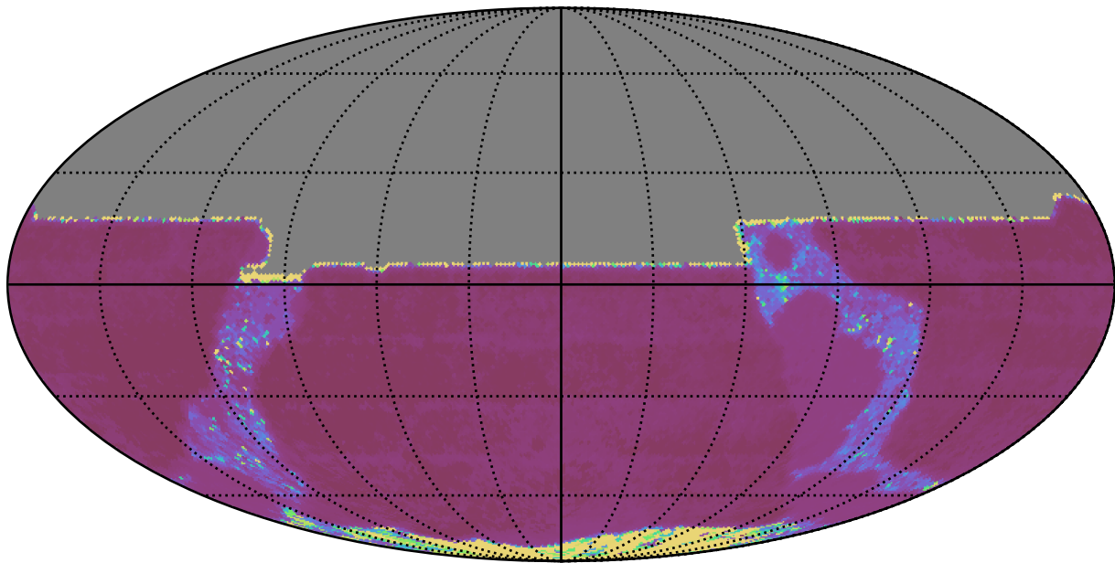
too_elab_r8_d3_giz_v3.4_10yrs All sky y band: Median Inter-Night Gap
