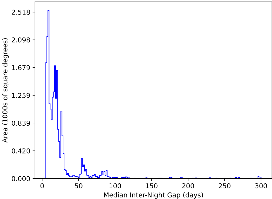
too_elab_r8_d3_giz_v3.4_10yrs All sky y band: Median Inter-Night Gap
