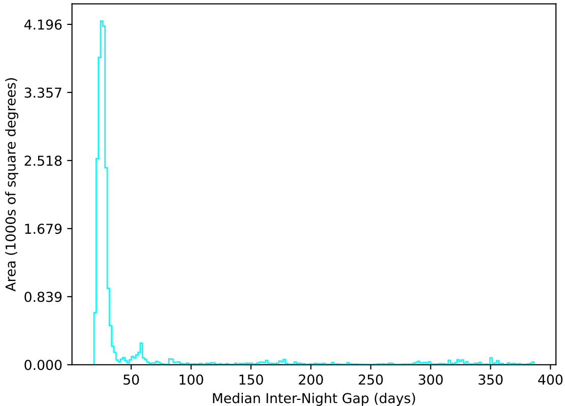
too_elab_r8_d3_giz_v3.4_10yrs All sky u band: Median Inter-Night Gap
