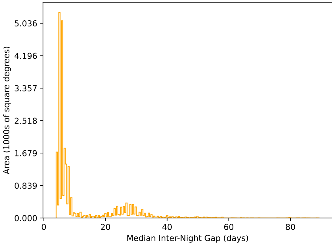
too_elab_r8_d3_giz_v3.4_10yrs All sky r band: Median Inter-Night Gap
