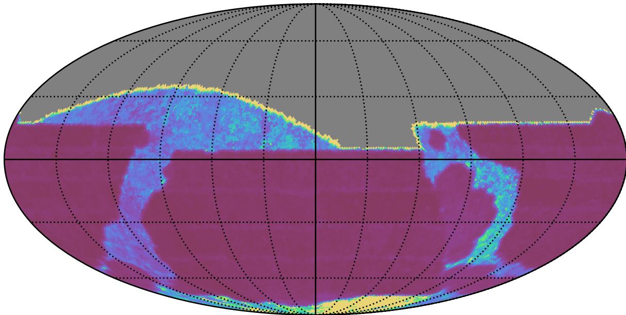
too_elab_r8_d3_giz_v3.4_10yrs All sky i band: Median Inter-Night Gap
