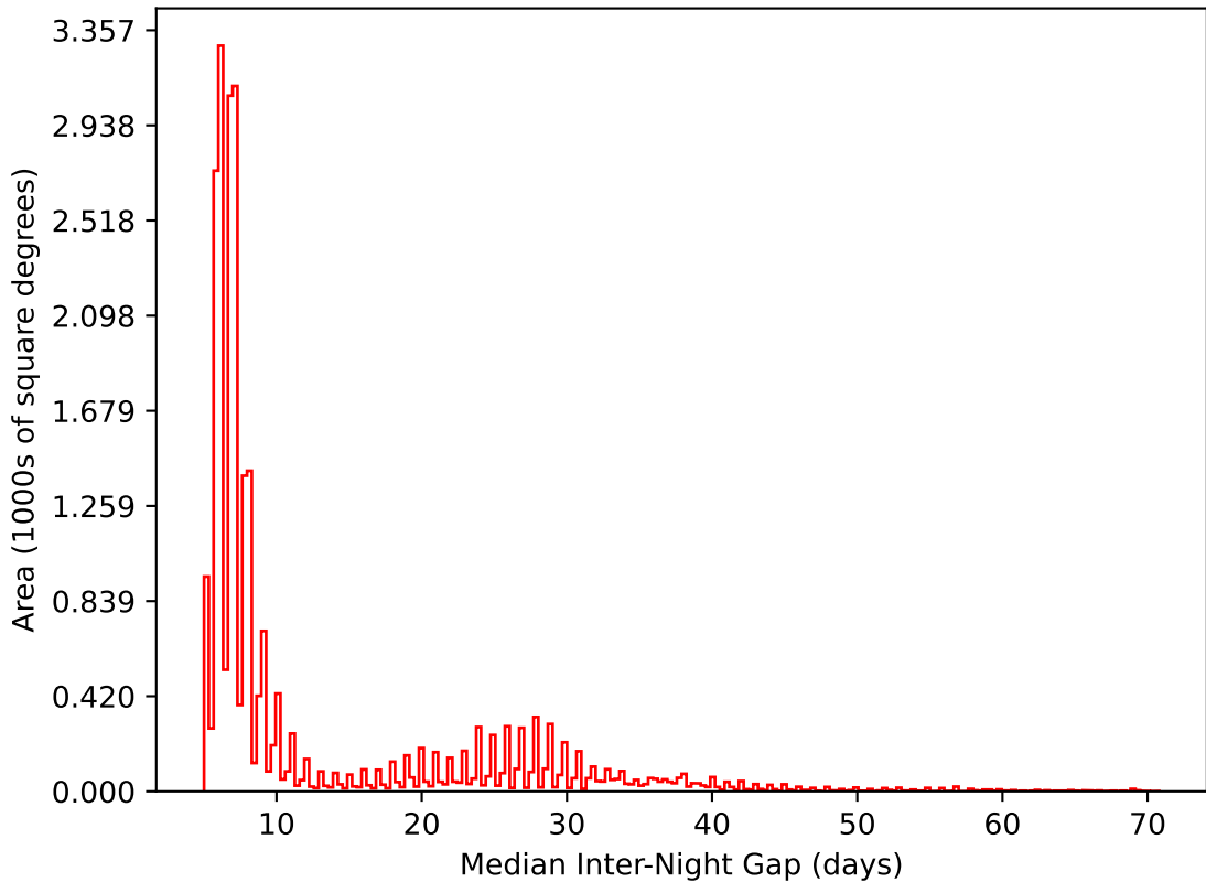
too_elab_r8_d3_giz_v3.4_10yrs All sky i band: Median Inter-Night Gap
