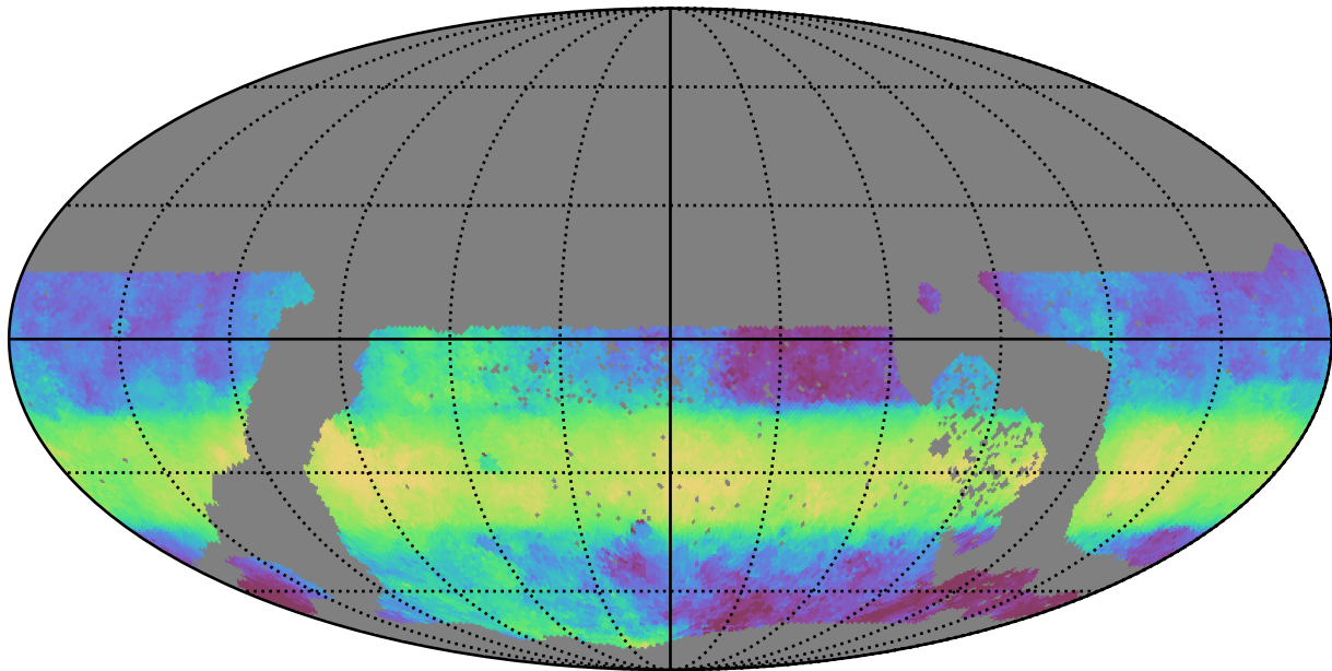
too_elab_r8_d3_giz_v3.4_10yrs WFD z band: Median HA
