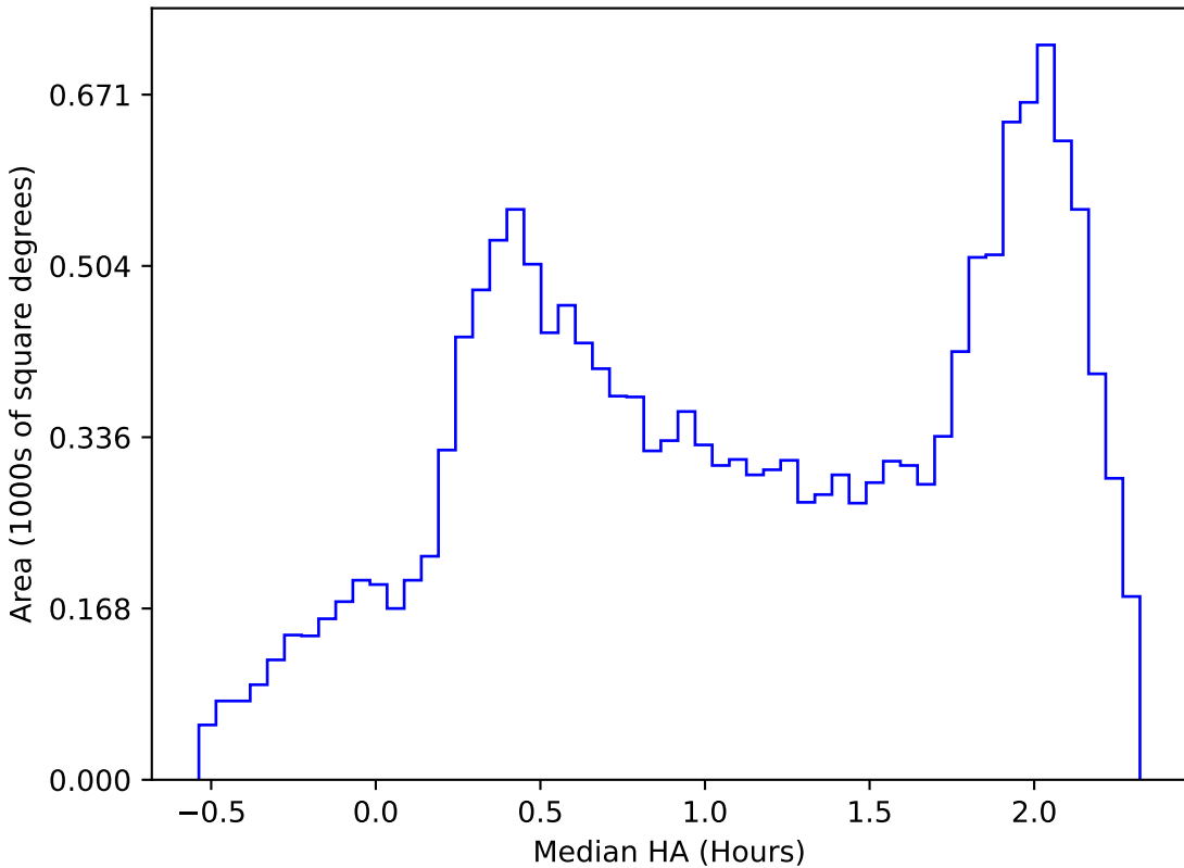
too_elab_r8_d3_giz_v3.4_10yrs WFD z band: Median HA
